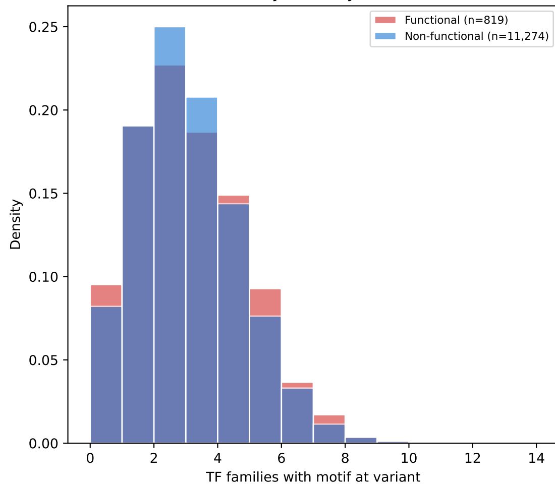
A. TF family diversity at variant
