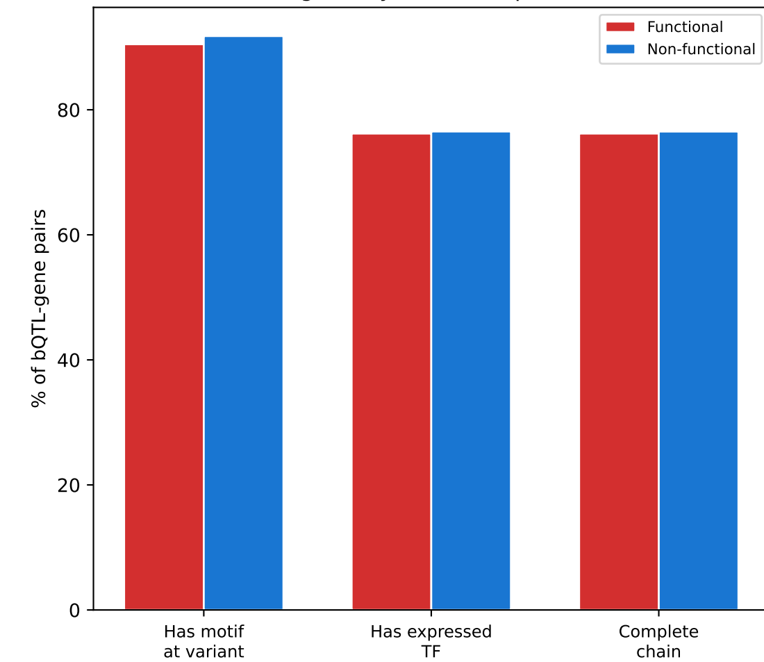
D. Regulatory chain completeness
