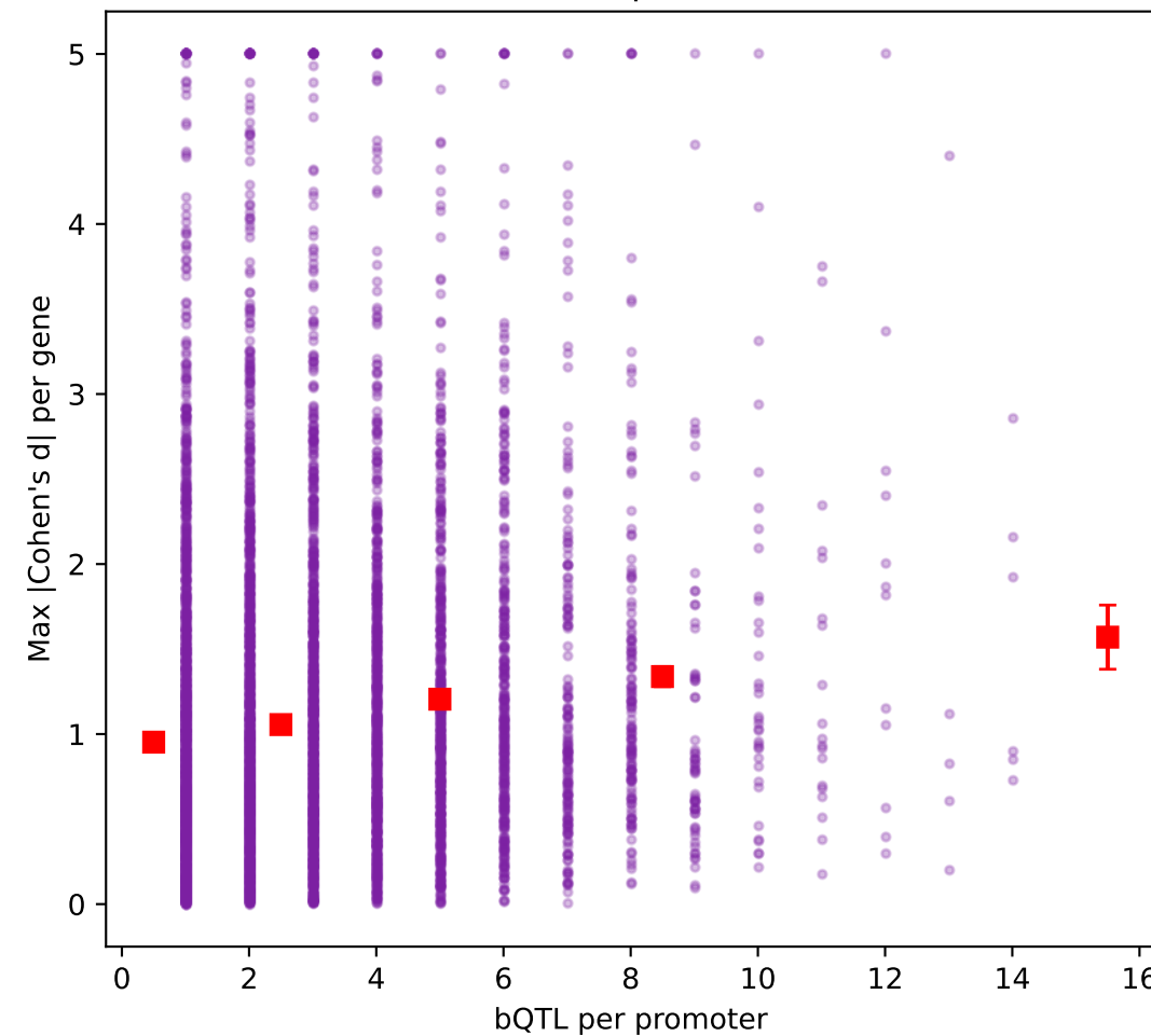
E. Promoter bQTL density vs effect \rho=0.153 , p=3.92e-38
