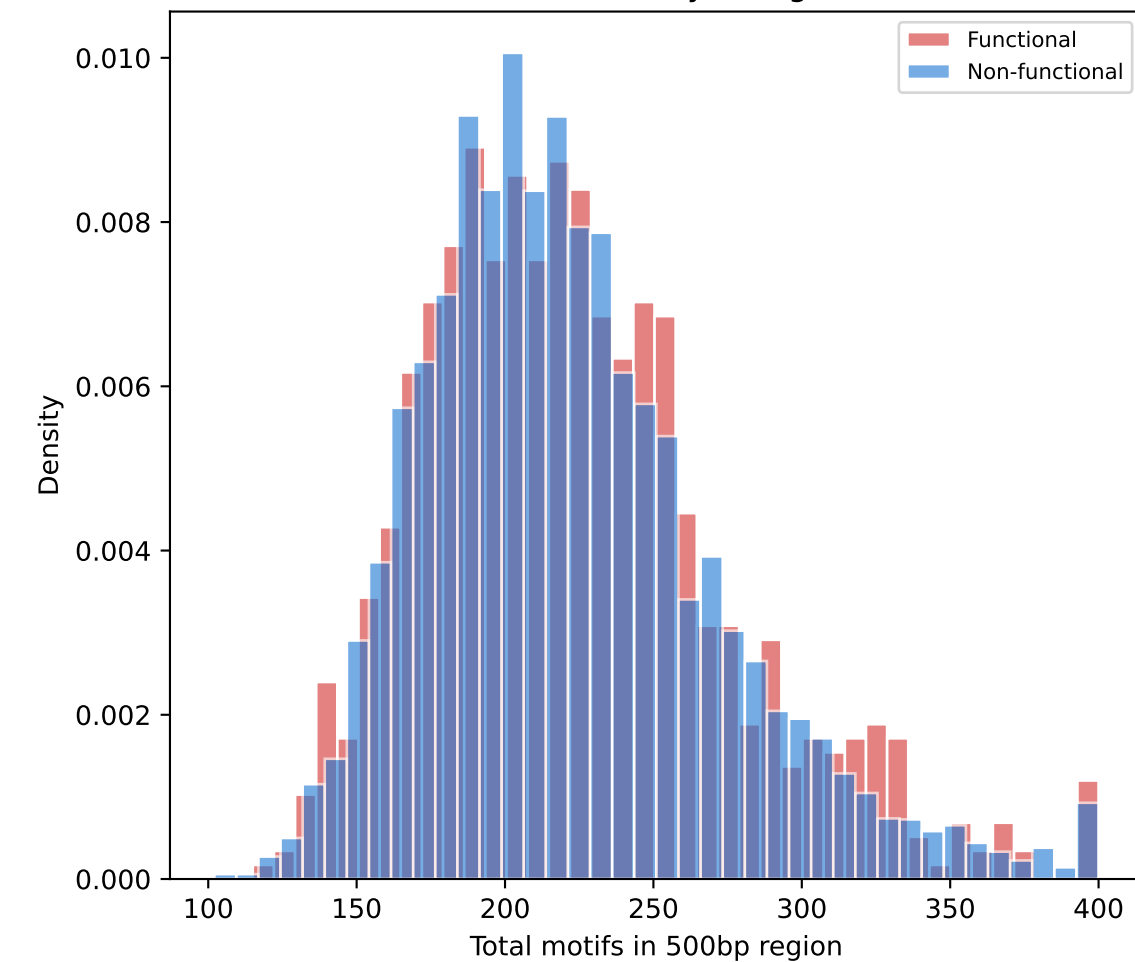
C. Motif density in region
