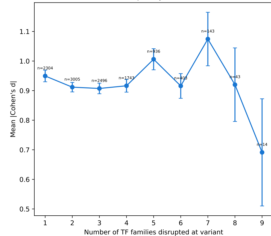
F. Motif complexity vs ASE effect
