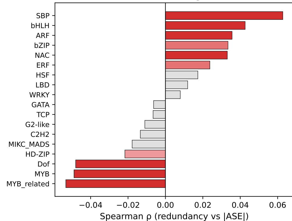
C. Per-family buffering effect (darker = more significant)
