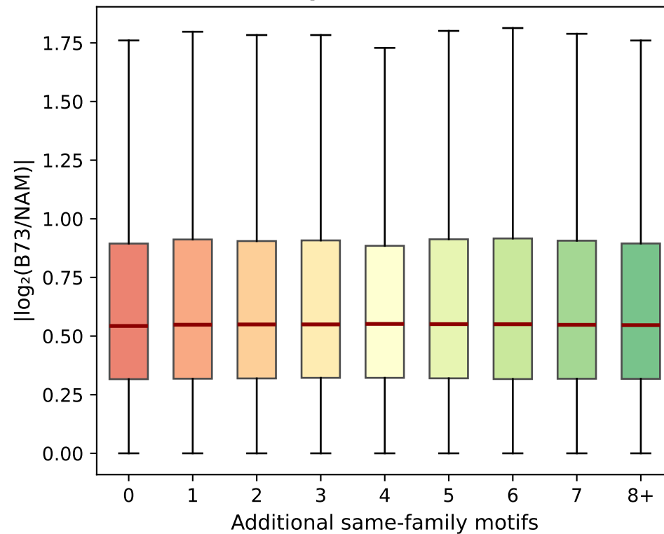
B. Redundancy vs allelic imbalance \rho = -0.004 ns
