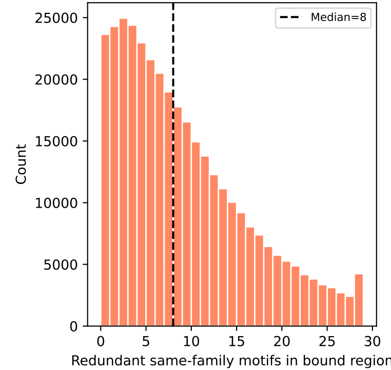
C. Within-region redundancy (sole: 6.3%)
