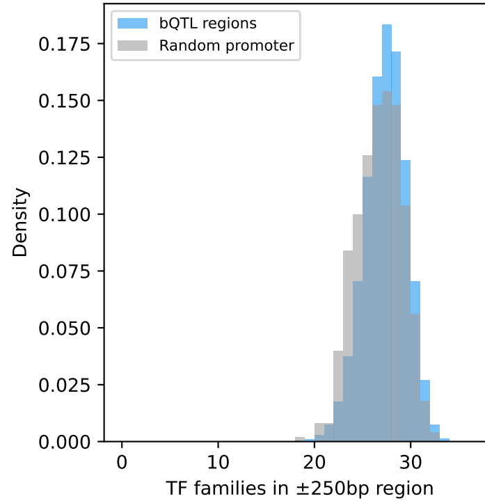
B. Family diversity: bQTL vs random
