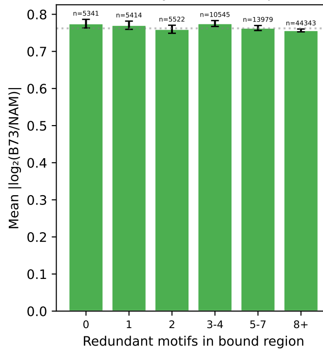
E. Redundancy vs allelic expression
