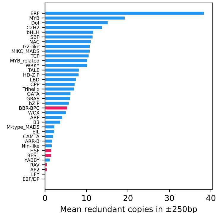
D. Per-family redundancy (red = >40\% sole)
