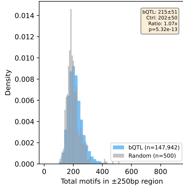
A. Motif density: bQTL vs random promoter
