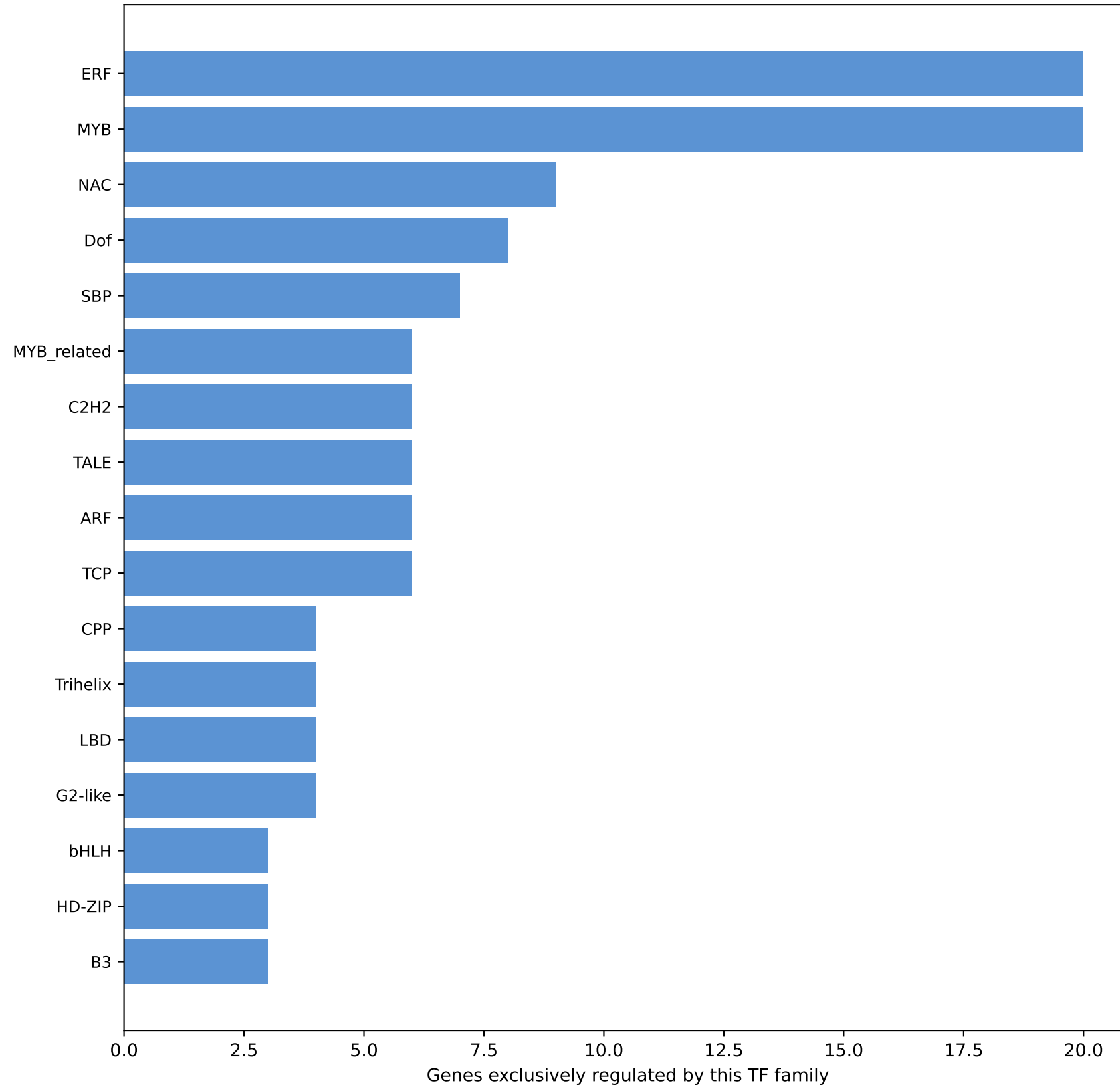
A. Sole-motif gene groups (only 1 TF family disrupted at bQTL)
