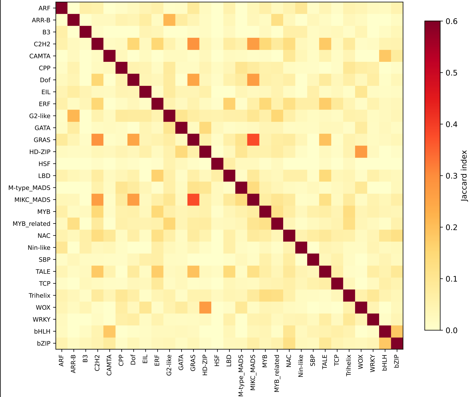
B. Jaccard overlap between TF family targets (do same genes have multiple motifs disrupted?)
