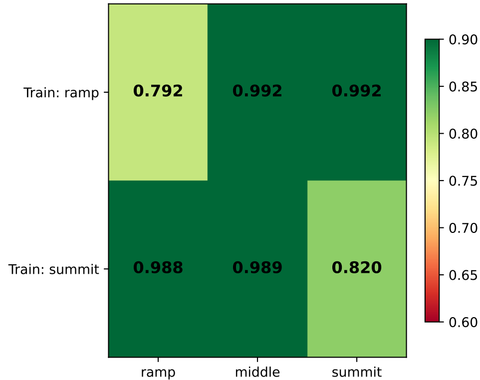
B. Cross-condition AUC
