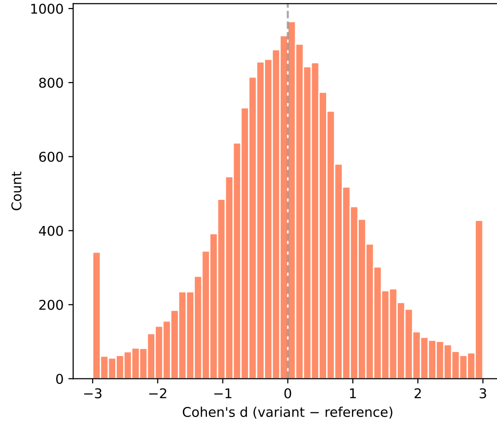
E. Group sizes median variant=6, ref=8
