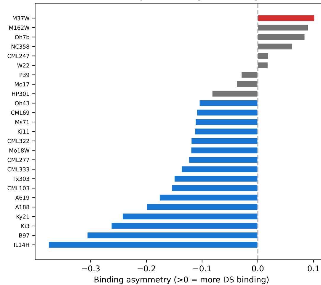
E. Per-hybrid binding remodeling
