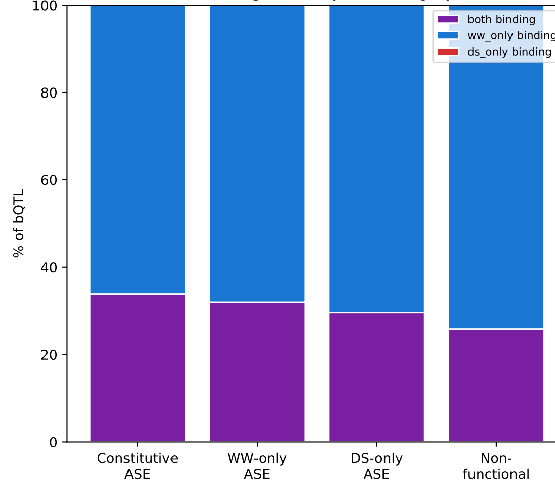
E. Per-hybrid binding remodeling
