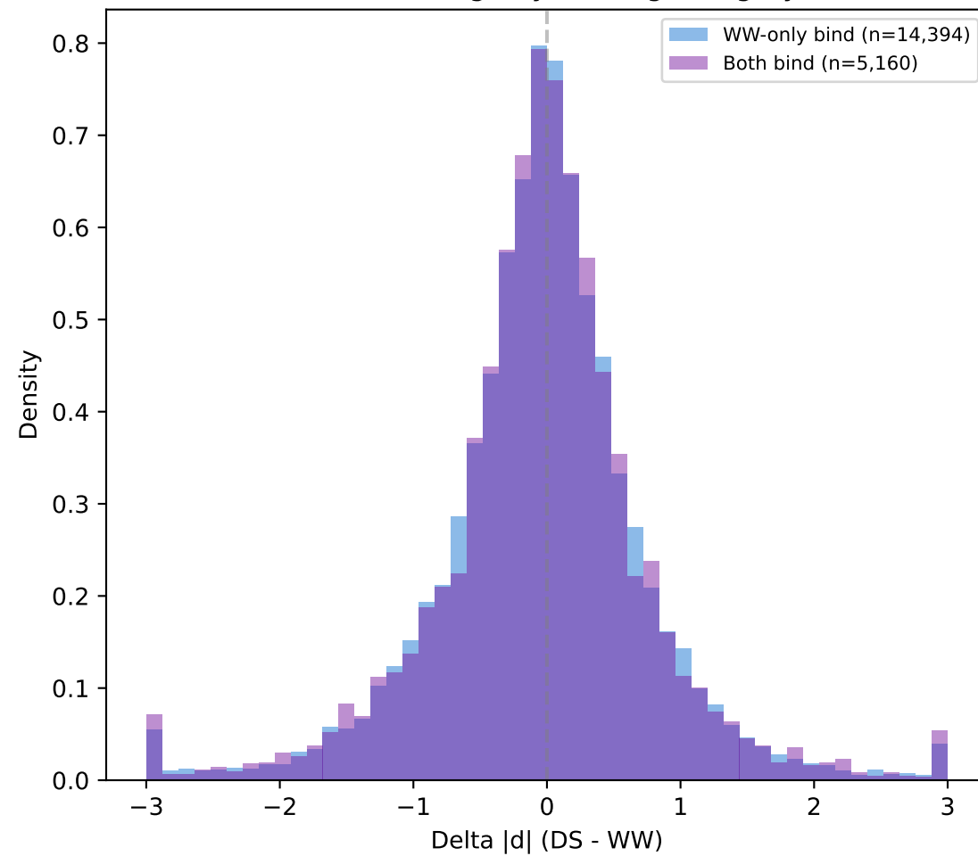
D. ASE change by binding category
