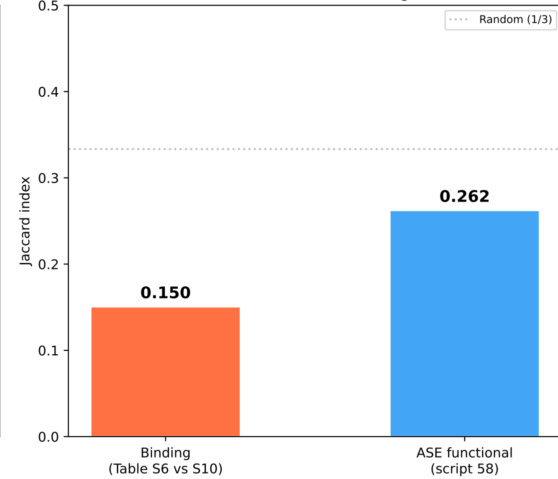
F. Condition overlap: binding vs ASE (lower = more switching)
