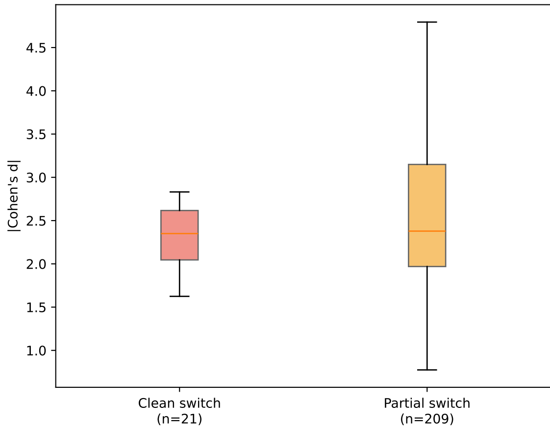
B. Clean vs partial sole-copy switches
