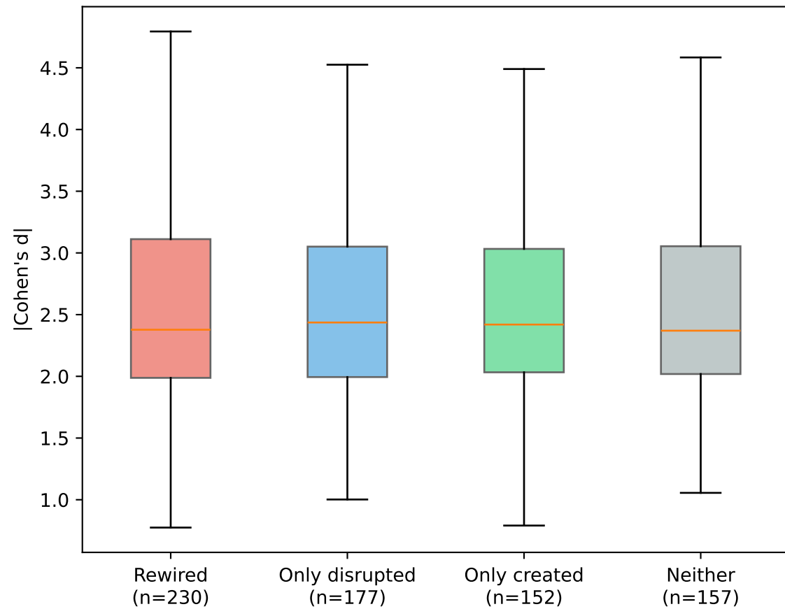
A. Effect size by motif change category
