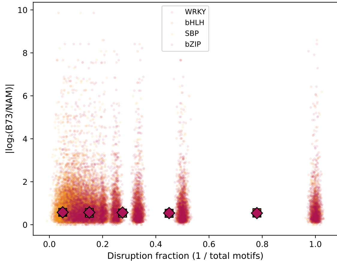
B. Sensitive families: disruption fraction vs ASE
