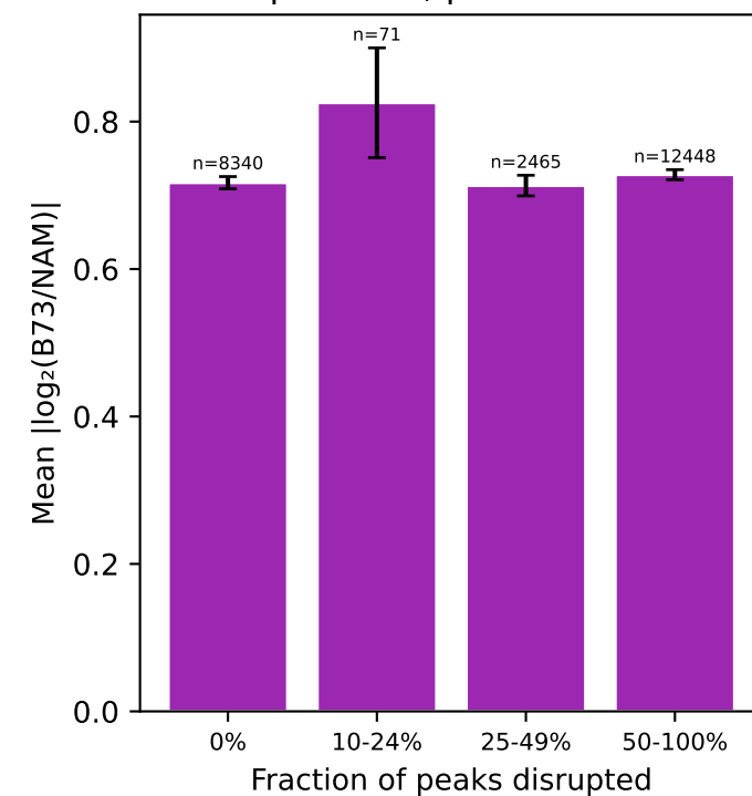
C. Fraction disrupted vs ASE \rho=0.014 , p=3.8e-02
