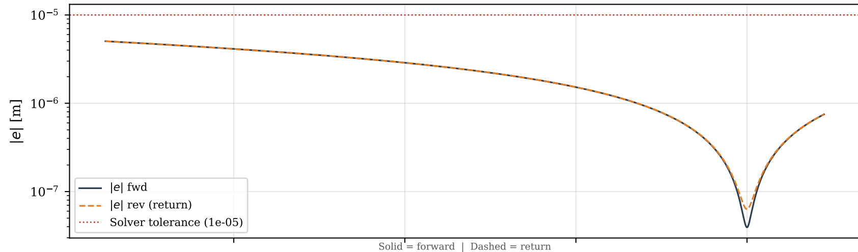
Closure residual vs \theta — forward and return sweeps overlap: residual is geometric, NOT accumulated
