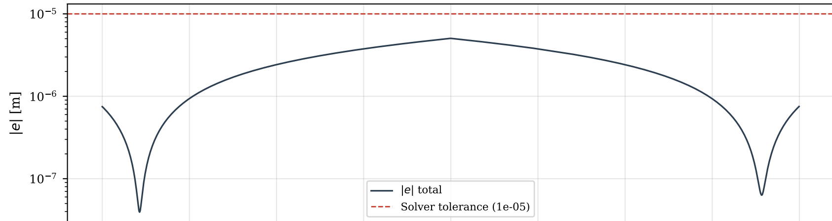
Kinematic closure residual vs simulation time
