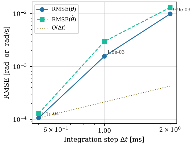
Trajectory accuracy vs \Delta t
