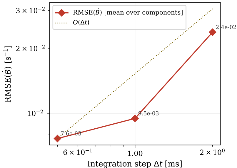
\dot{B}(q) FD approximation error vs \Delta t
