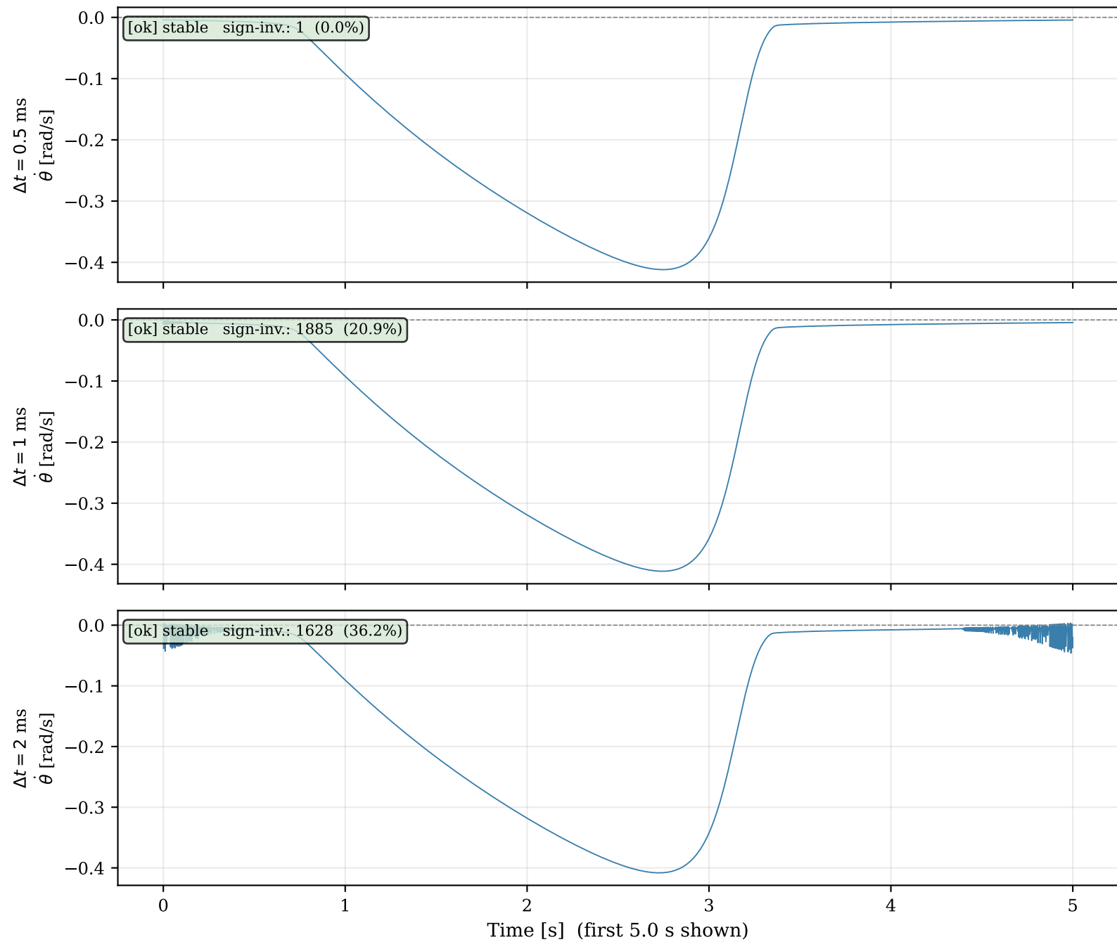
Integration stability: \dot{\theta}(t) at different \Delta t — \tau(t) = -|3.5||\sin(\pi t/10.0)| Nm
