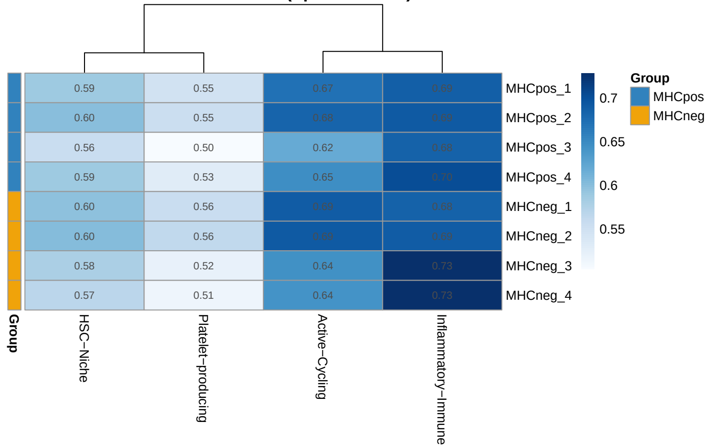
Bulk vs Sun subsets (Spearman rho)
