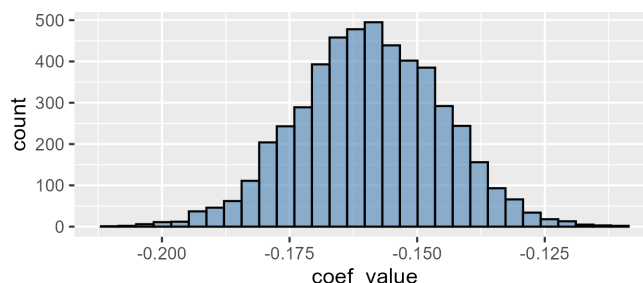
Figura 4. Coeficiente de female
