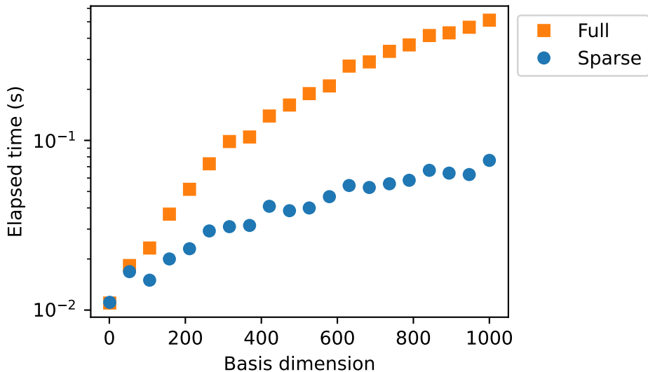
GaussianProduct, d=2 , n=1000
