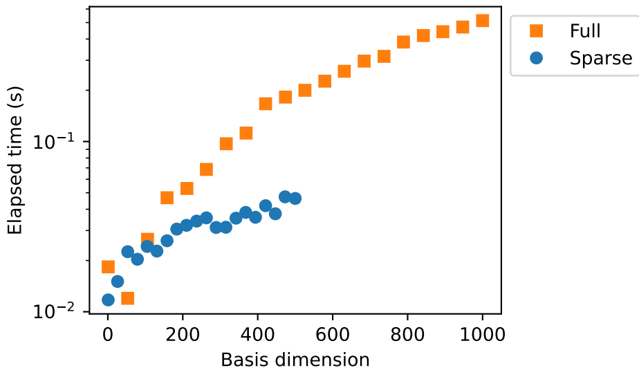
GaussianSum, d=2 , n=1000
