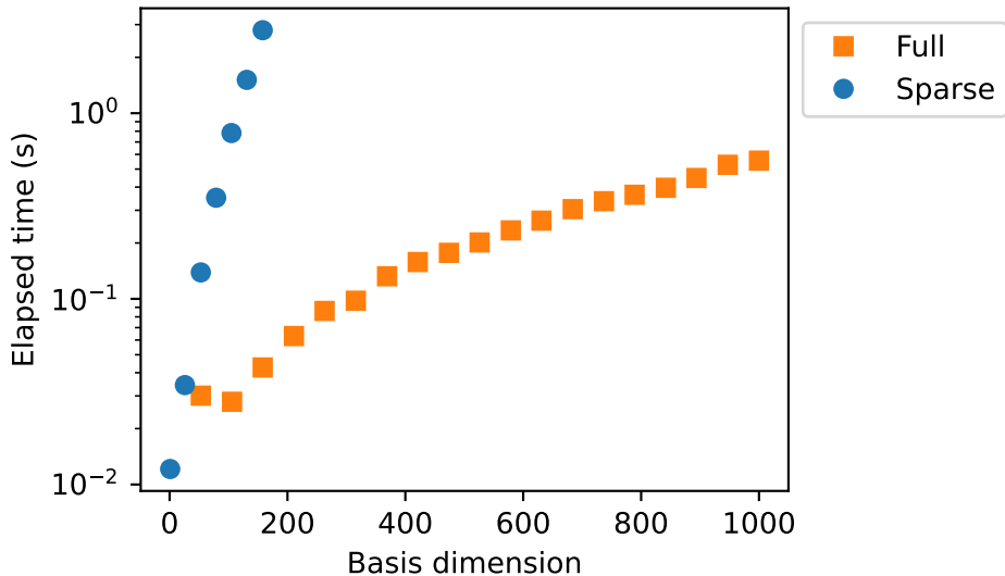
Oakley-O'Hagan, d=15 , n=1000
