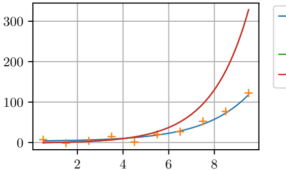
Exponential model.
