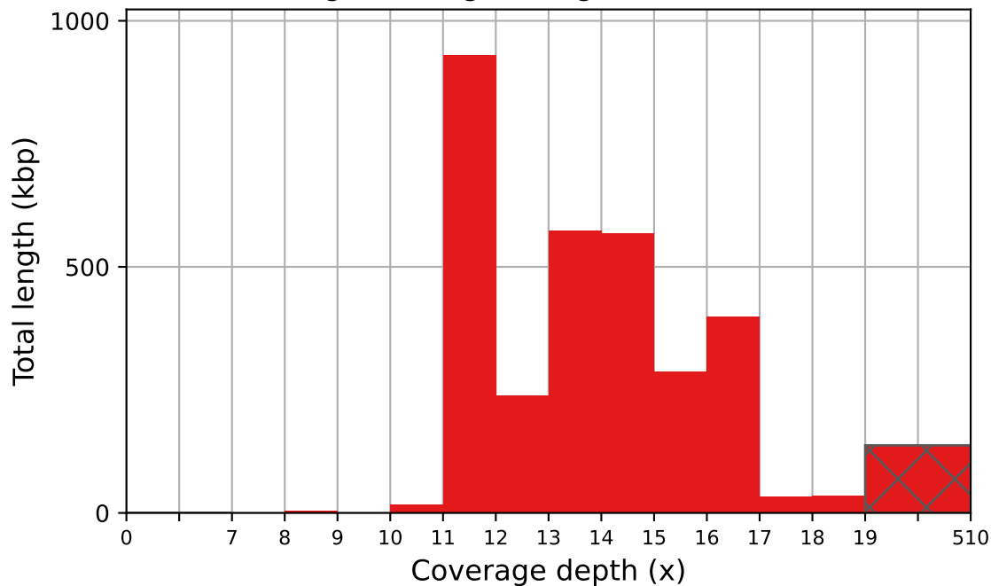
contigs coverage histogram (bin size: 1x)
