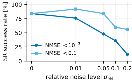
(b) SR success vs. noise
