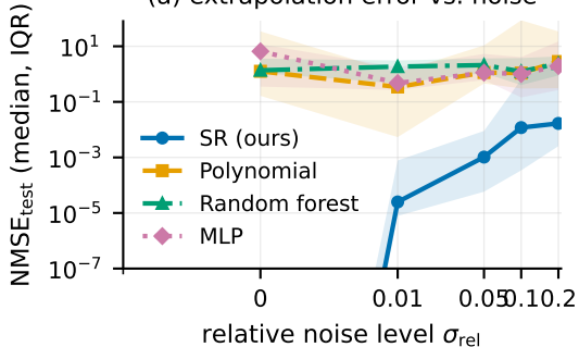
(a) extrapolation error vs. noise
