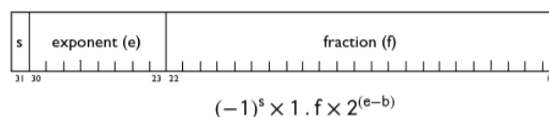
Figure 1: Diagram of IEEE-754 Floating-Point Representation
