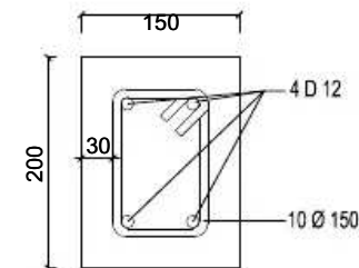
DETAIL RINGBALK SKALA 1 : 5
