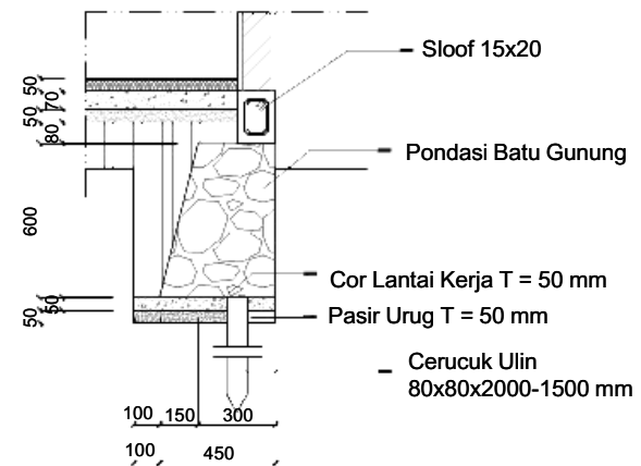
DETAIL B 1:20
