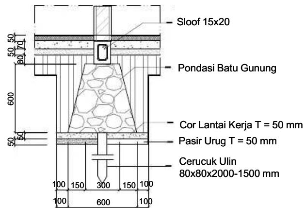
DETAIL A 1:20
