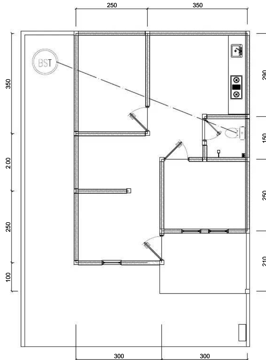
DENAH INSTALASI AIR KOTOR 1:50
