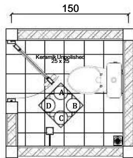
DENAH WC 1:30
