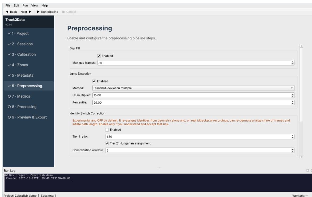
Figure 8. The Preprocessing screen with the default settings.
