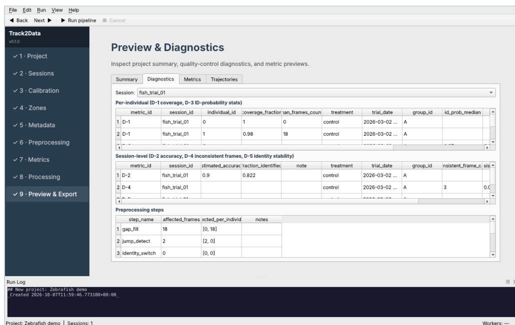
Figure 14. The Diagnostics tab.
