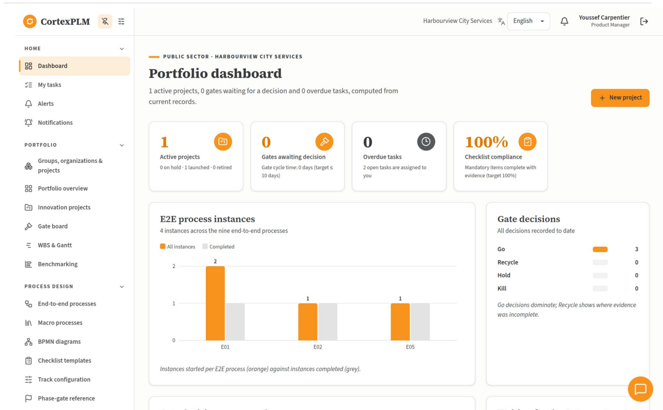
Dashboard of Harbourview City Services for its Product Manager, after Run 1.
