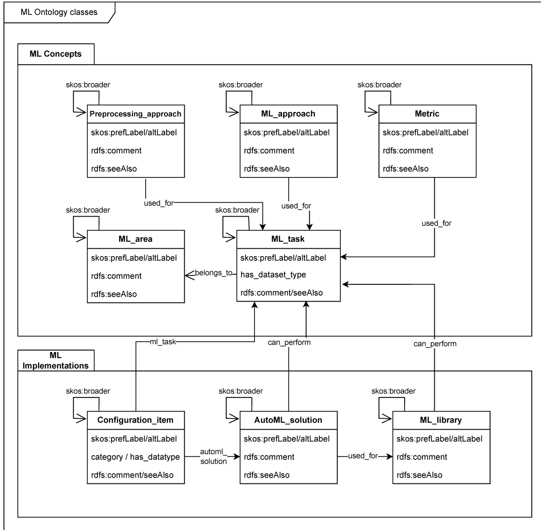
Figure 2.3.2: ML Ontology classes. Source: Humm (2026)
