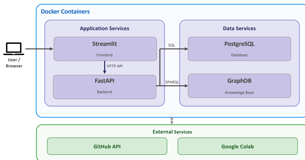
Figure 6.0.2: System Overview of MLguide
