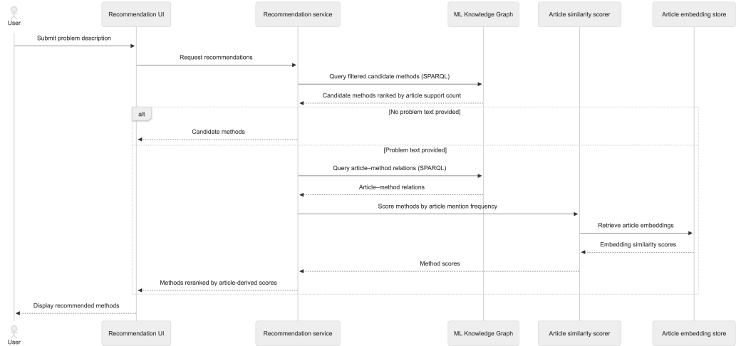
Figure 4.3.1: Sequence diagram of the recommendation process in MLguide.
