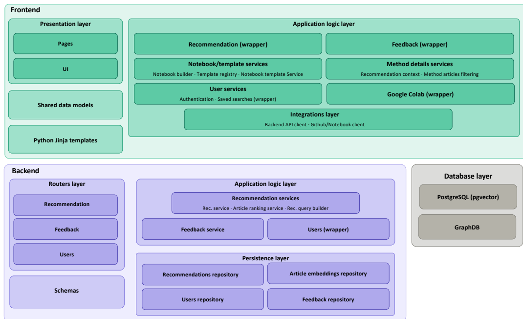
Figure 6.0.3: Package Diagram of MLguide
