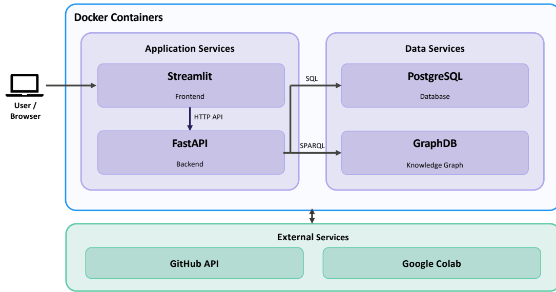
Figure 5.1.2: System Overview of MLguide
