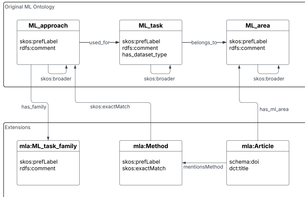
Figure 5.2.1: UML Class Diagram of the ML Ontology, including added classes and properties for MLguide
