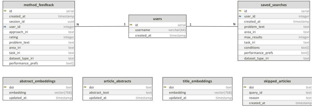
Figure 5.2.3: Entity-Relationship Diagram of the PostgreSQL database used in MLguide
