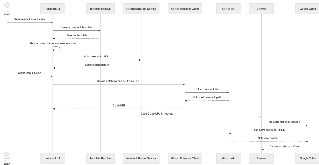
Figure 5.4.1: Sequence diagram of the notebook generation process in MLguide
