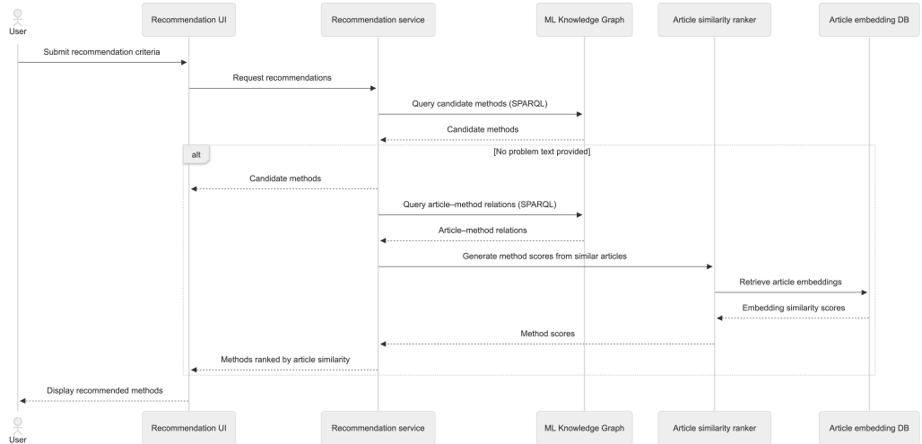
Figure 5.3.1: Sequence diagram of the article-based recommendation process in MLguide
