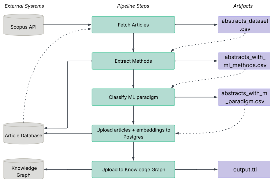
Figure 5.5.1: Flowchart of the article retrieval and knowledge extraction process in MLguide
