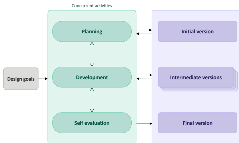
Figure 4.2.1: Illustration of the incremental development process, based on Sommerville (2011, p. 33)
