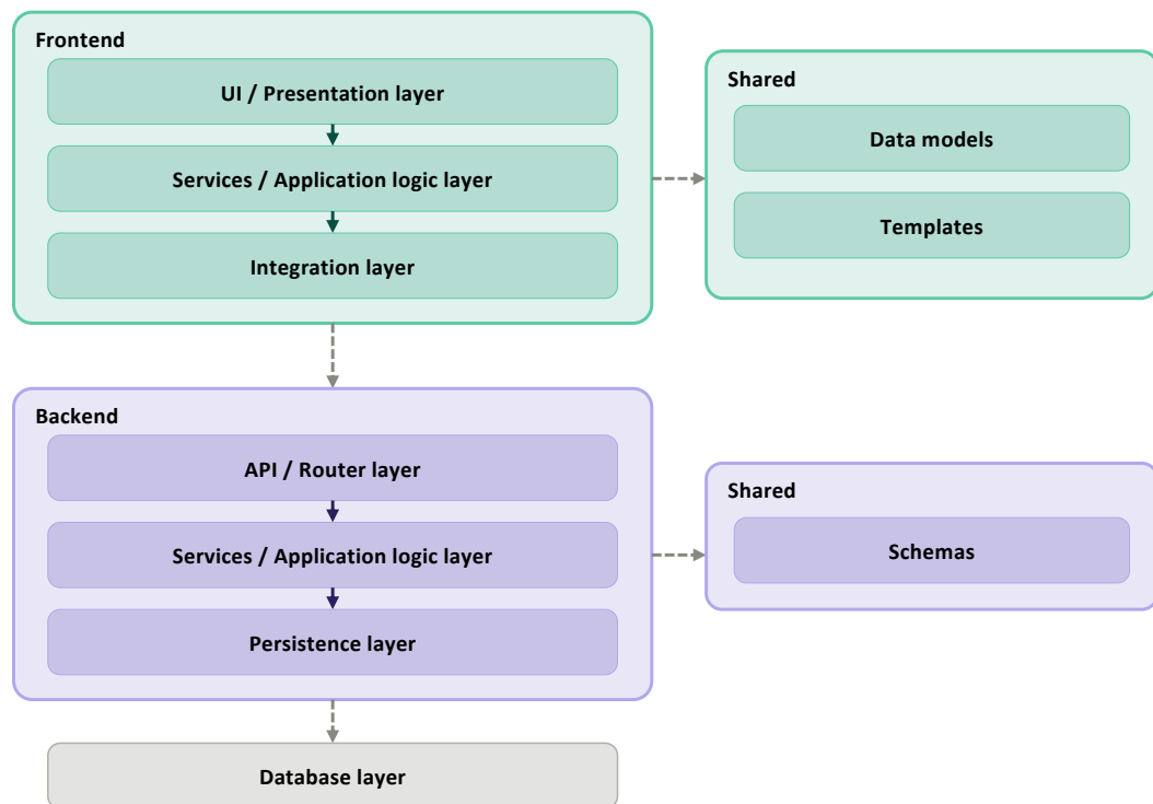
Figure 6.0.1: Layered Architecture of MLguide
