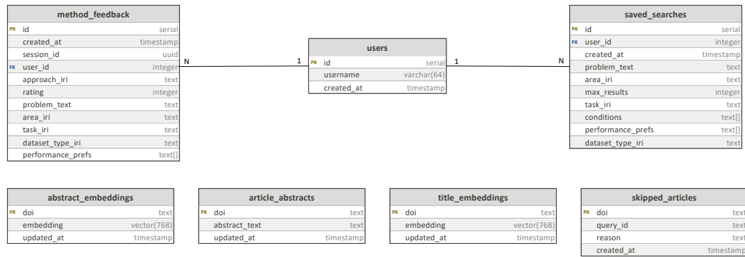
Figure 6.0.6: Entity-Relationship Diagram of the PostgreSQL database used in MLguide
