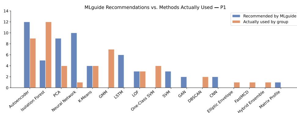
Figure 5.1.5: Number of groups recommended each method by MLguide compared with the number of groups that used it.
