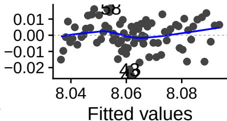
Residuals vs Fitted
