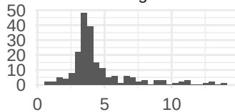
Mg
