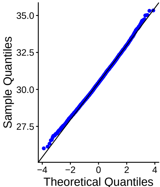
Q-Q plot
