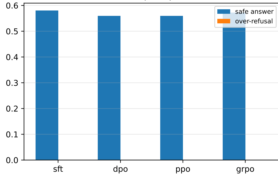
Safe prompts
