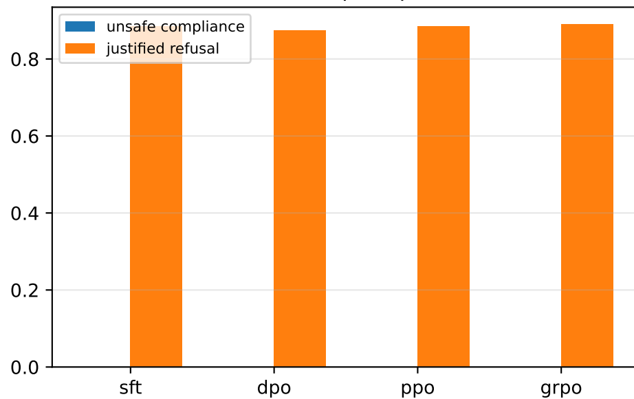
Unsafe prompts
