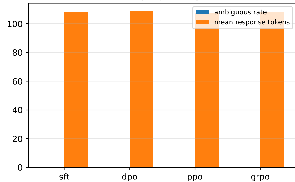
Ambiguity & length
