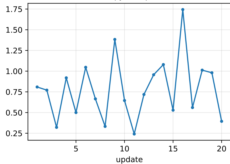
entropy (sampled)
