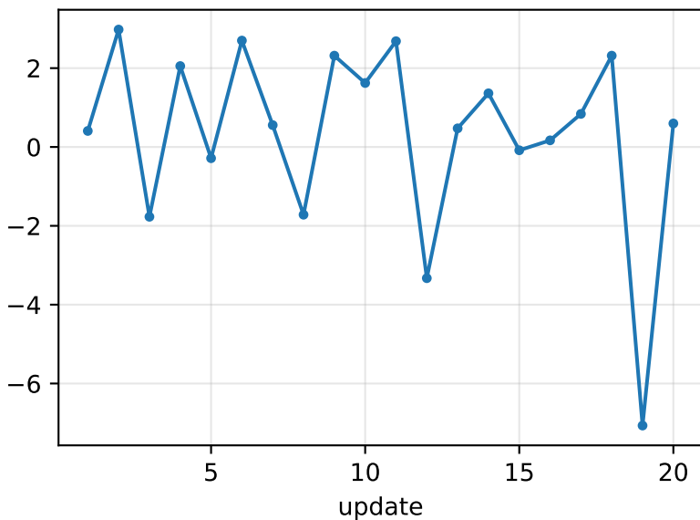
entropy (sampled)
