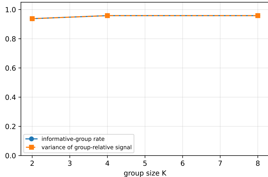
Equal-generation group-size study (overall)
