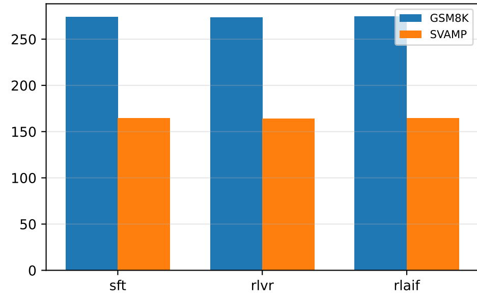
Mean response length
