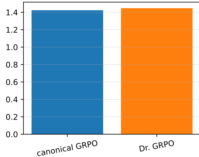
held-out reward
