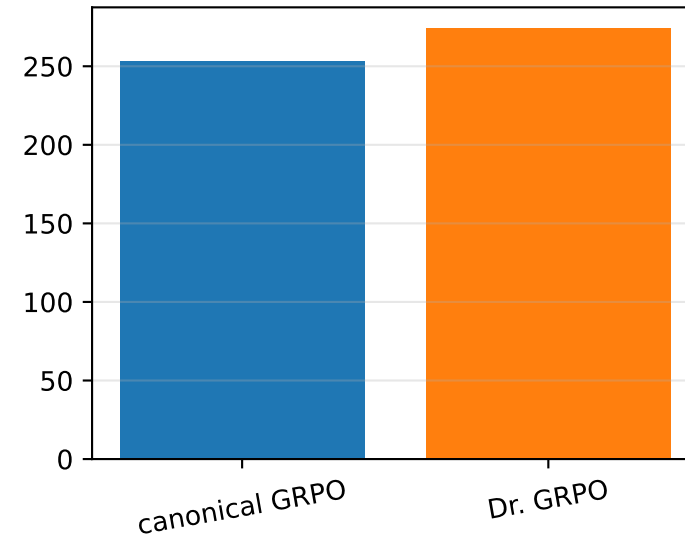
held-out length
