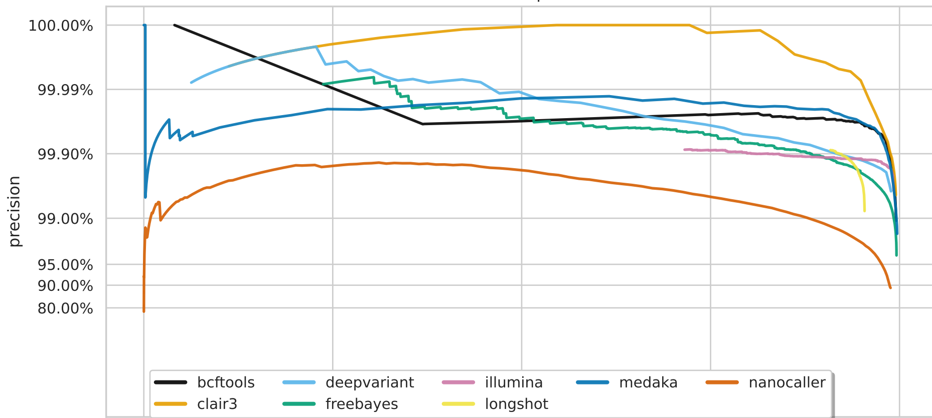
INDEL simplex
