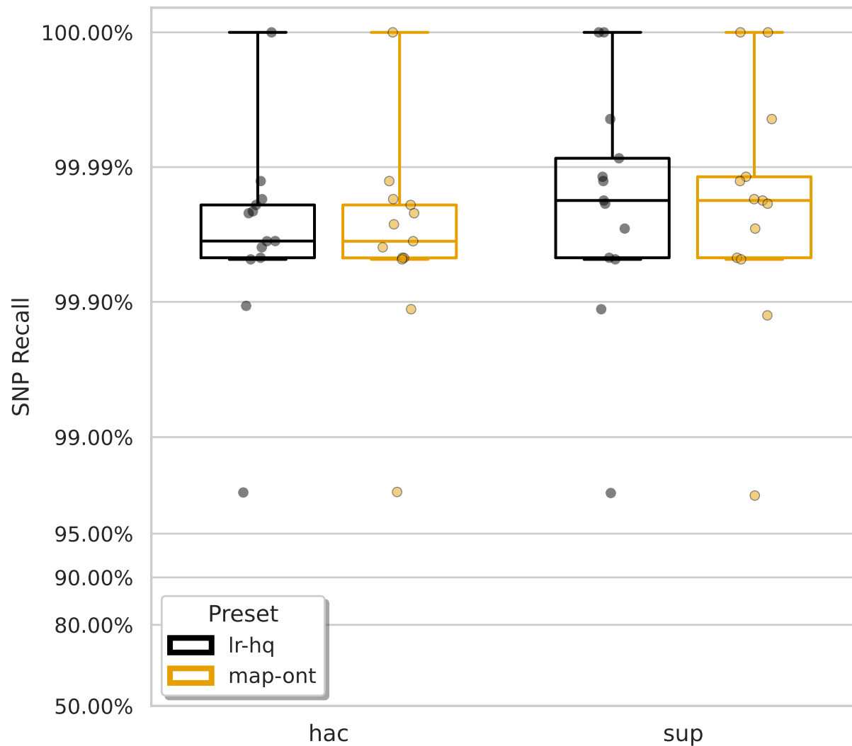
SNP Recall
