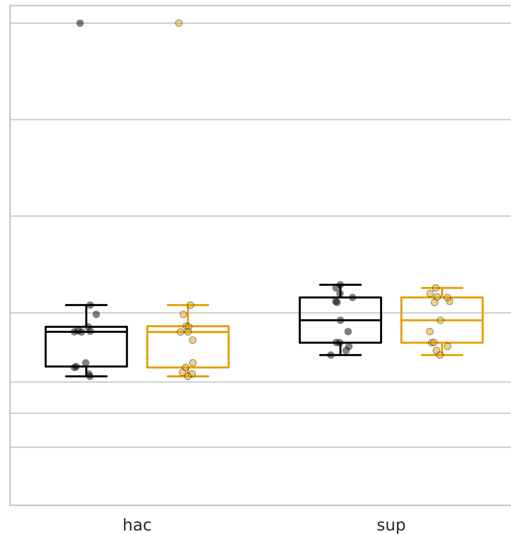
INDEL Recall
