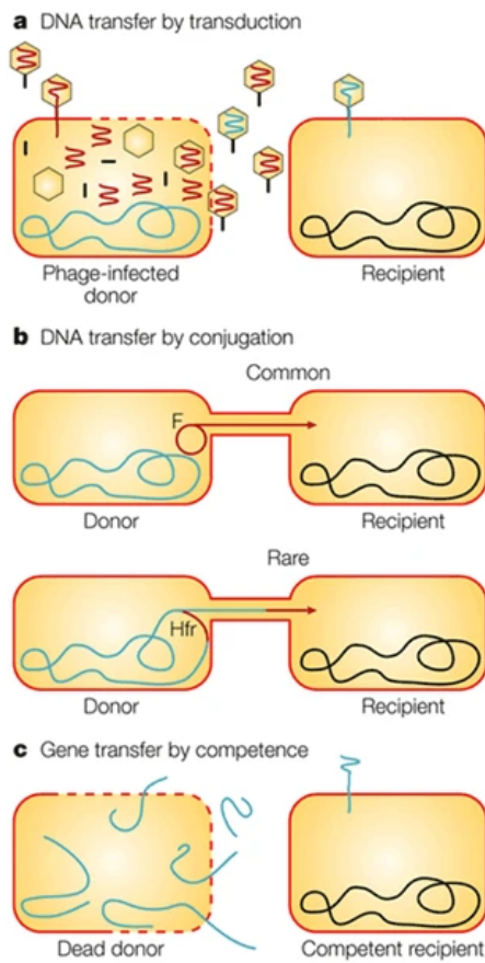
Fig. 1.1: An illustration of the three main mechanisms of horizontal inheritance in bacteria. a) Transduction is facilitated by phages that encapsulate host DNA in one cell and eject that DNA into another cell. b) Conjugation, in its prevalent form, is the transfer of a plasmid copy from a donor to a receiver cell via a pilus "bridge". In a rarer form, a plasmid that has been incorporated into the donor cell chromosome is transferred. c) Transformation (competence) is the uptake of exogenous DNA and subsequent incorporation into the chromosome.
