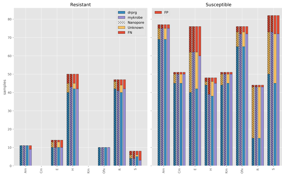
Fig. 4.8: Number of resistant (left) and susceptible (right) culture-based drug susceptibility testing (DST) phenotypes correctly identified by mykrobe (purple) and drprg (blue) with Illumina (non-striped) and Nanopore (striped) data. The red bars indicate missed (FN) or incorrect (FP) predictions. The yellow bars represent drprg "unknown" calls, which is when there is an off-panel variant found in a gene associated with the respective drug. If there is no resistance-associated variant found for that drug, then an unknown call is made. The x-axis shows the drugs with available phenotype data. E - ethambutol; H - isoniazid; R - rifampicin; S - streptomycin; Km - kanamycin; Am - amikacin; Ofx - ofloxacin; Cm - capreomycin.
