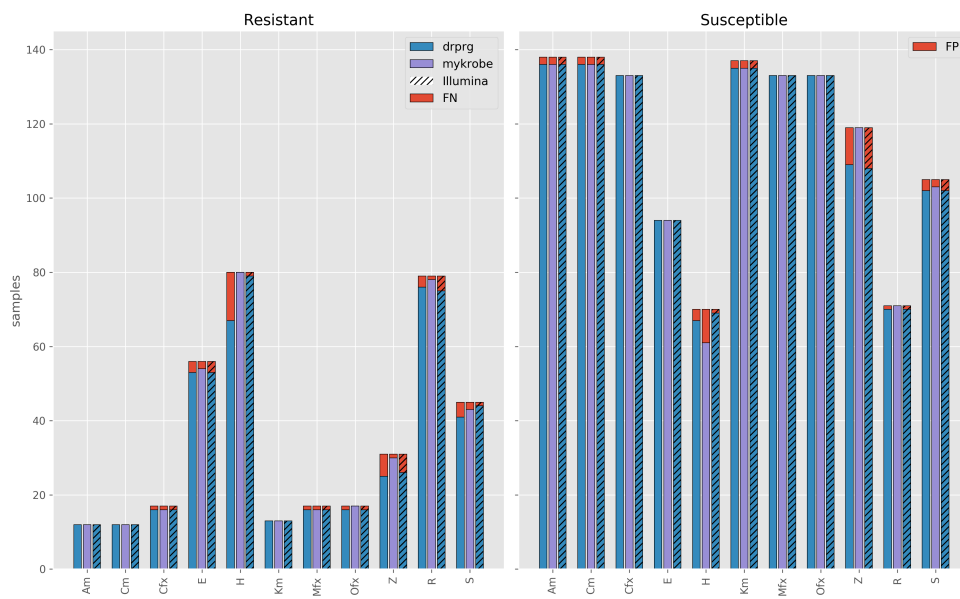
Fig. 4.4: Number of resistant (left) and susceptible (right) WGS-based drug resistance phenotypes correctly identified by mykrobe Nanopore (purple) and drprg (blue) with Illumina (striped) and Nanopore (non-striped) data. For this analysis, the Illumina-based mykrobe predictions are considered truth and the other predictions are assessed accordingly. The red bars indicate missed (FN) or incorrect (FP) predictions. The x-axis shows the drugs for which mykrobe makes predictions. E - ethambutol; H - isoniazid; Z - pyrazinamide; R - rifampicin; S - streptomycin; Km - kanamycin; Am - amikacin; Ofx - ofloxacin; Cm - capreomycin; Mfx - moxifloxacin.
