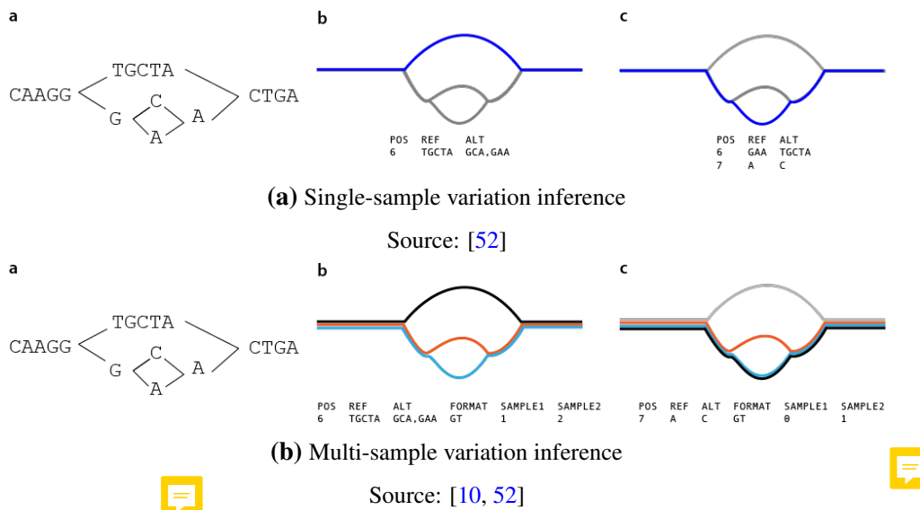
Fig. 1.6: The impact of sequence inference on variant representation. In both (a) and (b) the left panel (a) shows the PRG. (a) the blue line indicates the inferred sequence (maximum likelihood path). b and c show how the choice of this sequence affects the representation of variant sites when genotyping. (b) the black line indicates the multi-sample inferred sequence, while the blue and orange lines are two different samples. b and c show that small differences between the samples are represented as small variants by inferring the sequence that is maximally close to the two samples (c).
