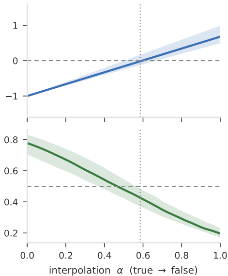
qwen2.5-0.5b 128 decisive paths
