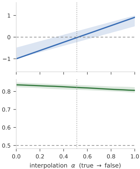
pythia-410m 0 decisive paths
