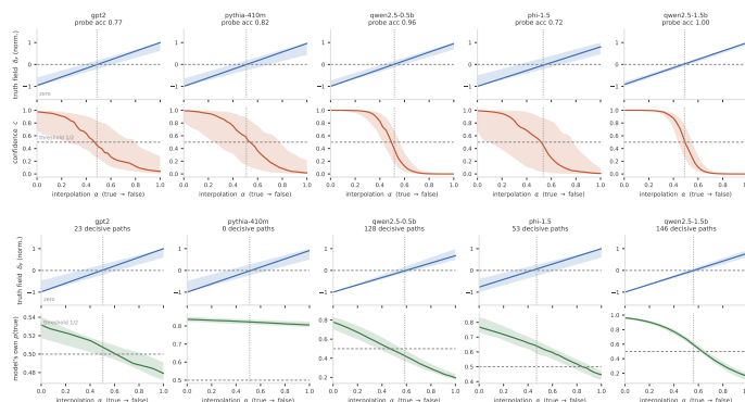
Figure 2: Upper pair of rows, the truth probe (normalized, median and interquartile band) and the independently trained confidence along true-to-negation paths, the dotted line marking the mean probe zero crossing where confidence passes one half in every model. Lower pair, the same with the model’s own probability of answering true from patched final-block states, decisive paths only. The Qwens sweep through one half at the boundary, Pythia-410M answers true everywhere so the premise fails, and GPT-2 and Phi-1.5 sit between.
