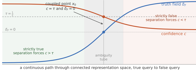
Figure 1: The coupling theorem in one picture. Along any true-to-false path, separation forces confidence above \tau on the strictly true side and below on the strictly false side, so both fields must cross, and the crossings coincide at the coupled point x_0 inside the ambiguity tube of Theorem 12.
