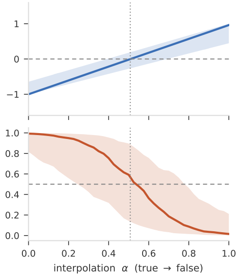
Pythia-410M probe acc 0.82
