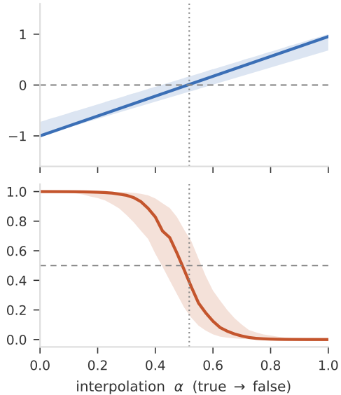
Qwen2.5-0.5B probe acc 0.96
