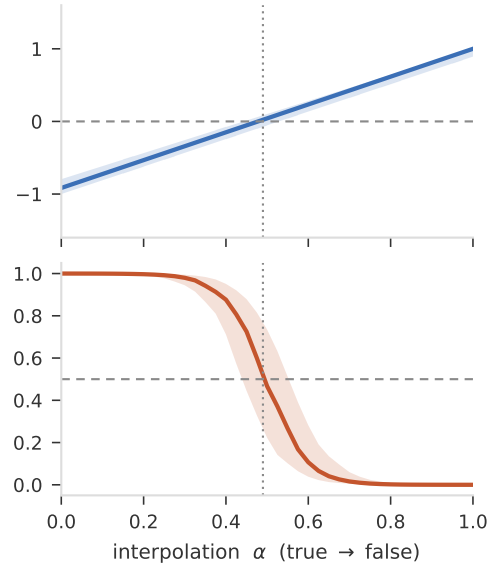
Qwen2.5-1.5B probe acc 1.00
