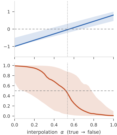
Phi-1.5 (1.3B) probe acc 0.72
