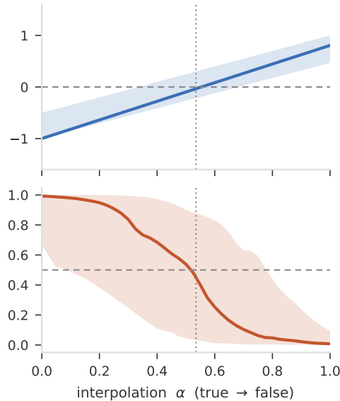
phi-1.5 probe acc 0.72
