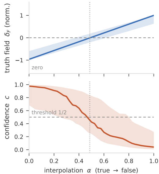
gpt2 probe acc 0.77
