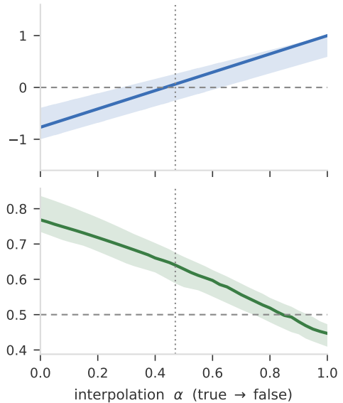
phi-1.5 53 decisive paths
