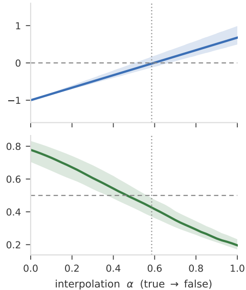
qwen2.5-0.5b 128 decisive paths
