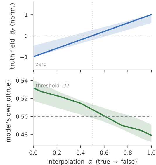
gpt2 23 decisive paths
